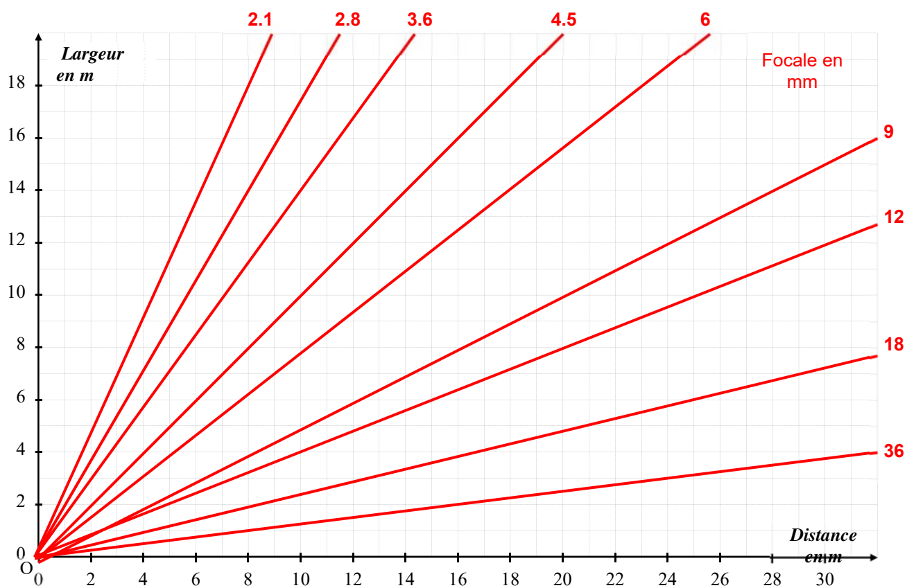
Abaque distance focale
