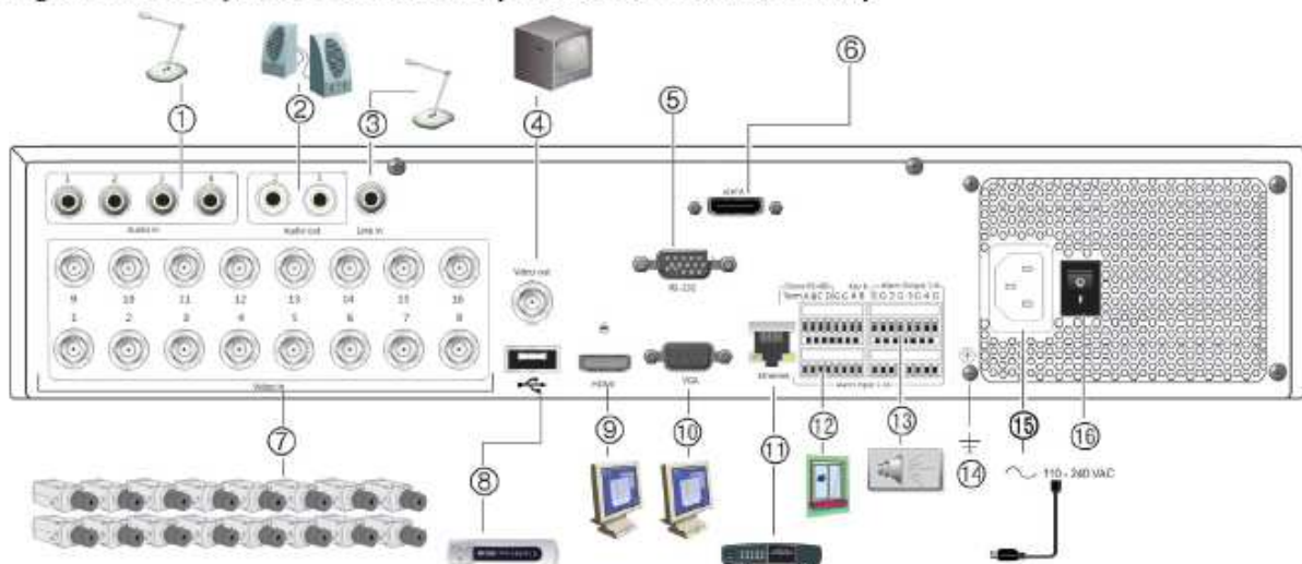
Figure 1: Back panel connections (16-channel model shown)
