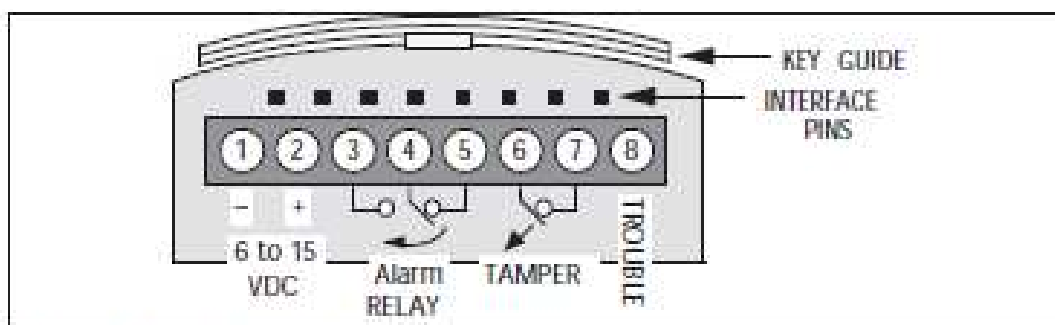
Figure 3.1: Wiring to terminals
